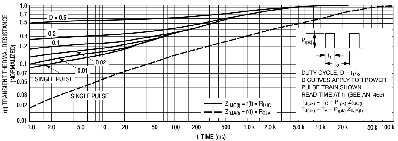
Figure 5. Thermal Response
