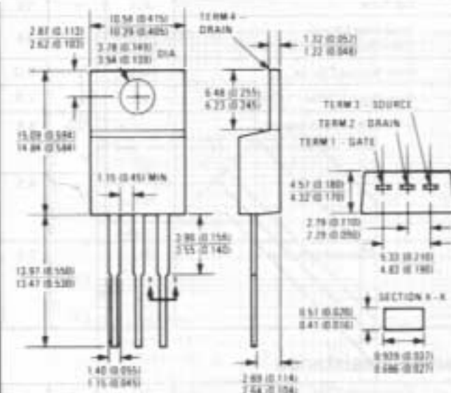
Case Style TO-220AB All Dimensions in Millimeters and (Inches)
