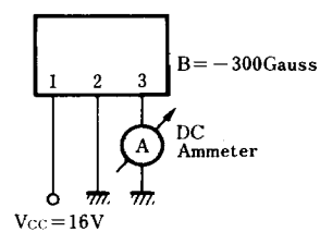
Test Circuit 4 ( -I_{OS} )
