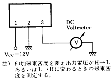
Test Circuit 1 ( B_{(1)} , B_{(2)} )
