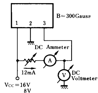
Test Circuit 2 ( V_{OL} )
