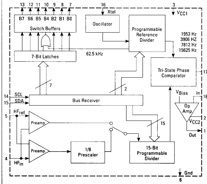
SIMPLIFIED BLOCK DIAGRAM
