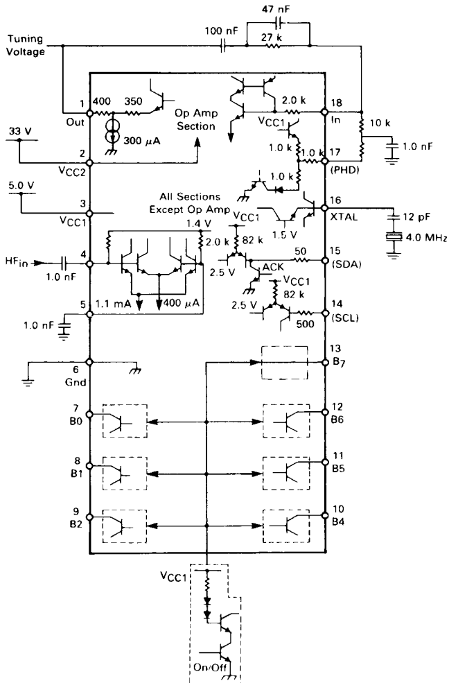
FIGURE 3 — PIN CIRCUIT SCHEMATIC
