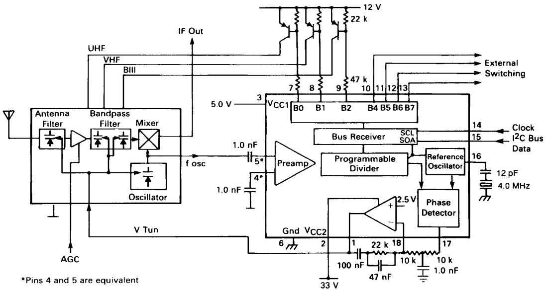
FIGURE 5 — TYPICAL TUNER APPLICATION
