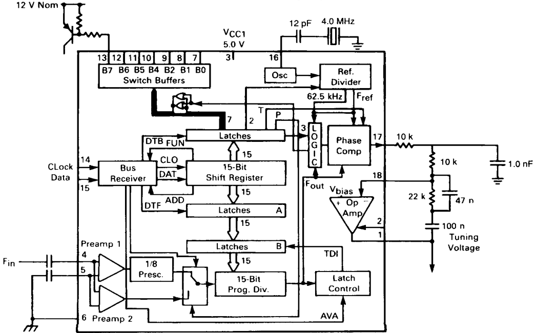
FIGURE 5 — TYPICAL TUNER APPLICATION
