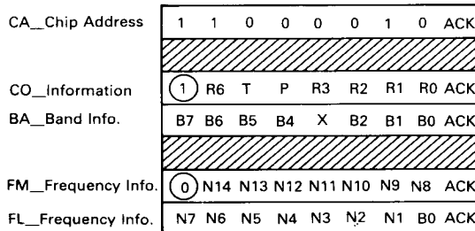
FIGURE 6 — DEFINITION OF BYTES
