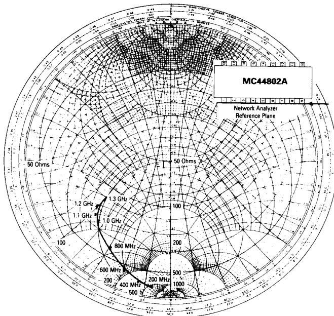
FIGURE 2 — PIN 5 INPUT IMPEDANCE (TYP)
