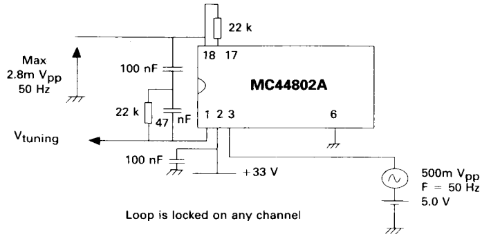
FIGURE 1b — HF SENSITIVITY TEST CIRCUIT
