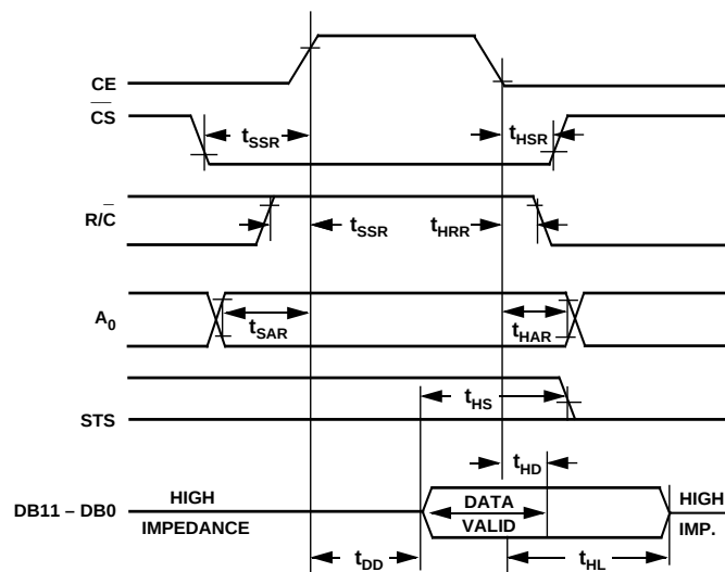
Figure 2. Read Timing
