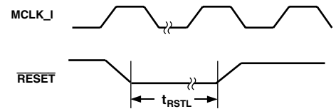
Figure 2. \overline{\text{RESET}} Timing
