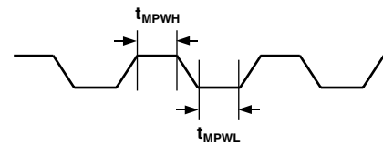
Figure 3. MCLK_I Timing
