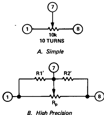
Figure 1. Nulling Circuits
