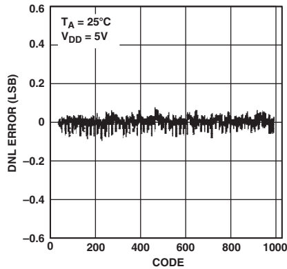
TPC 5. AD5312 Typical DNL Plot
