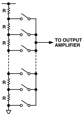
Figure 28. Resistor String
