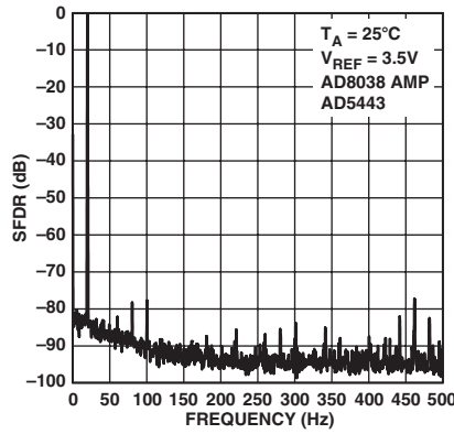
TPC 32. Wideband SFDR f_{OUT} = 20\text{ kHz} , Update = 1 MHz
