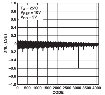
TPC 6. DNL vs. Code (12-Bit DAC)
