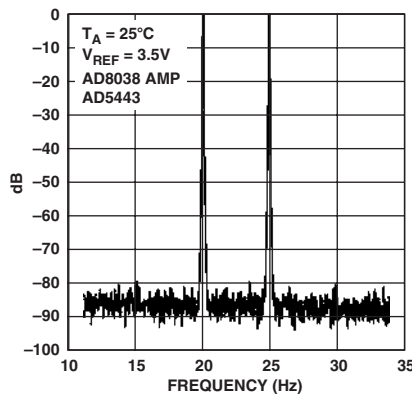
TPC 35. Narrowband ( \pm 50\% ) IMD, f_{OUT} = 20\text{ kHz} , 25 kHz, Update = 1 MHz
