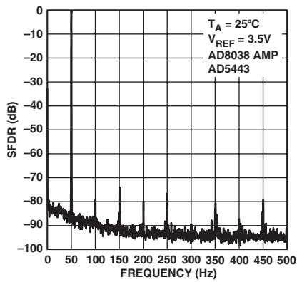
TPC 31. Wideband SFDR f_{OUT} = 50\text{ kHz} , Update = 1 MHz
