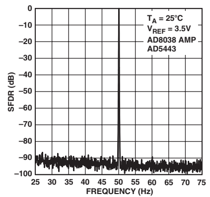
TPC 33. Narrowband ( \pm 50\% ) SFDR f_{OUT} = 50\text{ kHz} , Update = 1 MHz
