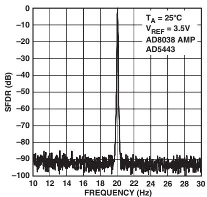
TPC 34. Narrowband ( \pm 50\% ) SFDR f_{OUT} = 20\text{ kHz} , Update = 1 MHz
