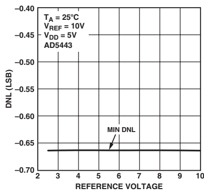
TPC 8. DNL vs. Reference Voltage
