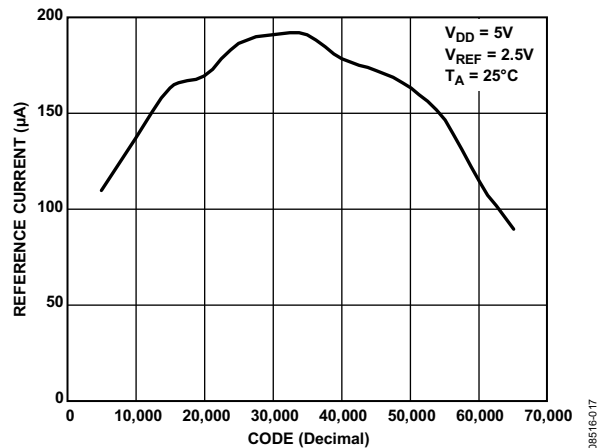
Figure 18. Reference Current vs. Code
