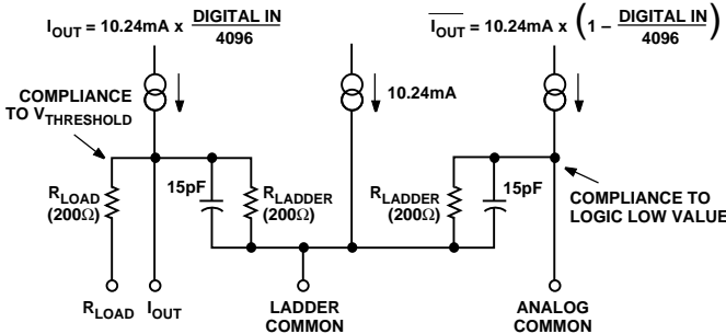
Figure 11. Equivalent Output
