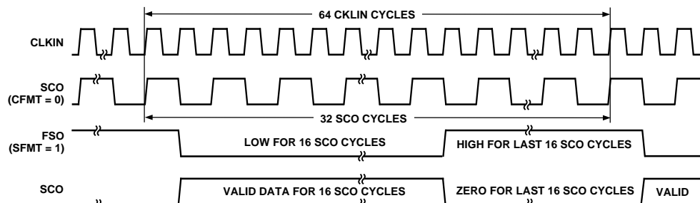
Figure 2b. Generalized Serial Mode Timing ( FSI = \text{Logic Low or High} , TSI = \text{DOE} )
