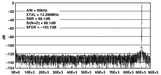
Figure 23. 16K Point FFT
