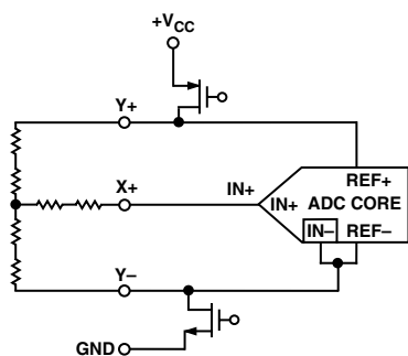
Figure 7. Differential Reference Mode ( SER/DFR = 0 )
