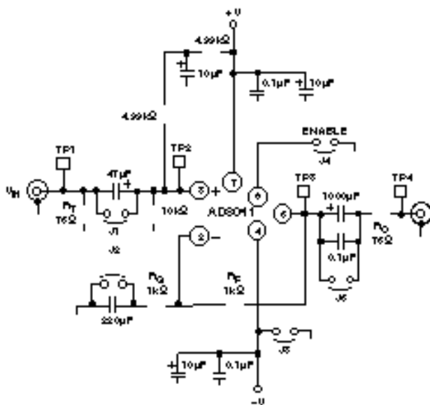
Figure 45. Noninverting Configurations for Evaluation Boards
