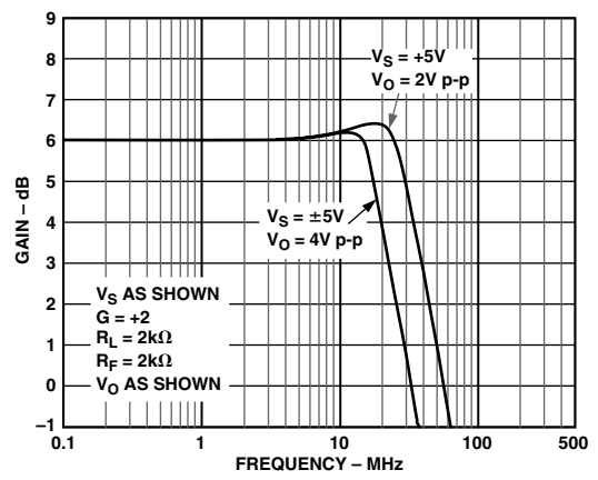
TPC 11. AD8054 Large Signal Frequency Response; G = +2
