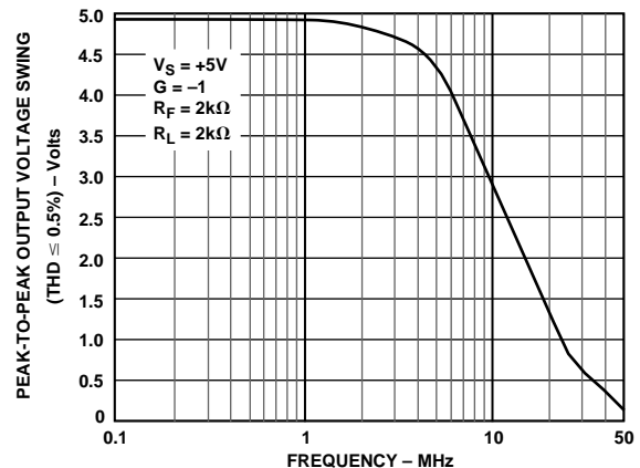
Figure 1. Low Distortion Rail-to-Rail Output Swing
