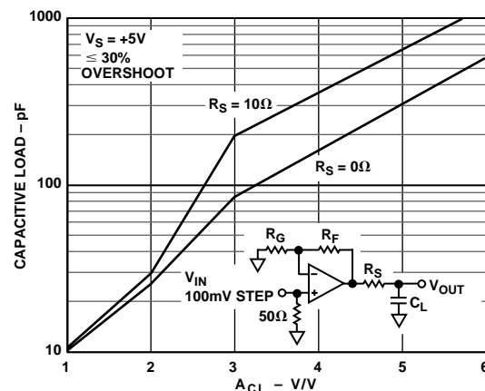
Figure 40. AD8054 Capacitive Load Drive vs. Closed-Loop Gain
