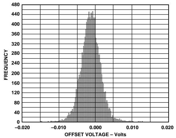
Figure 40. AD8111 Offset Voltage Distribution (RTI)
