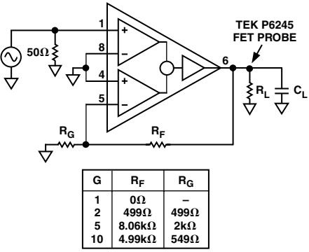
TPC 18. AD8130 Basic Frequency Response Test Circuit
