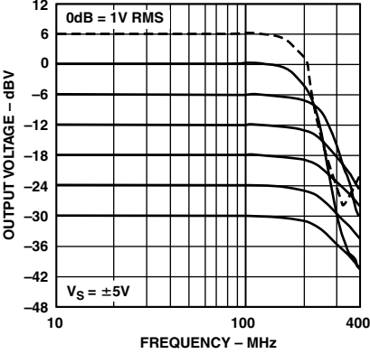
TPC 17. AD8130 Frequency Response for Various Output Levels
