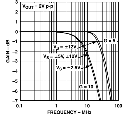
TPC 15. AD8130 Frequency Response vs. Supply, G = 5 , G = 10 , V_{OUT} = 2 \text{ V p-p}
