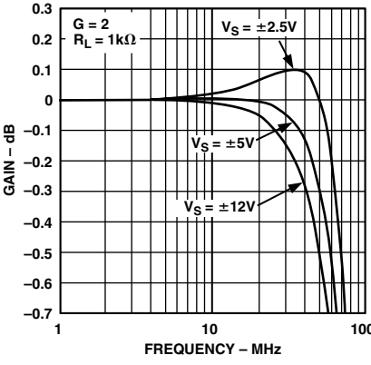
TPC 11. AD8130 Fine Scale Response vs. Supply, G = 2 , R_L = 1 \text{ k}\Omega
