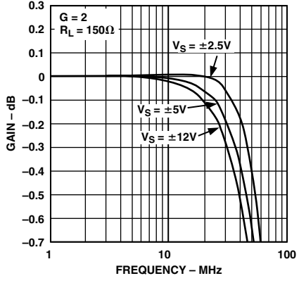
TPC 12. AD8130 Fine Scale Response vs. Supply, G = 2 , R_L = 150 \Omega
