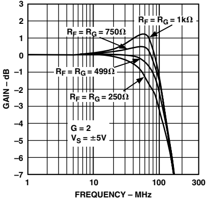
TPC 10. AD8130 Frequency Response for Various R_F/R_G
