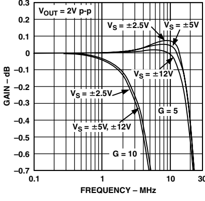
TPC 14. AD8130 Fine Scale Response vs. Supply, G = 5 , G = 10 , V_{OUT} = 2 \text{ V p-p}
