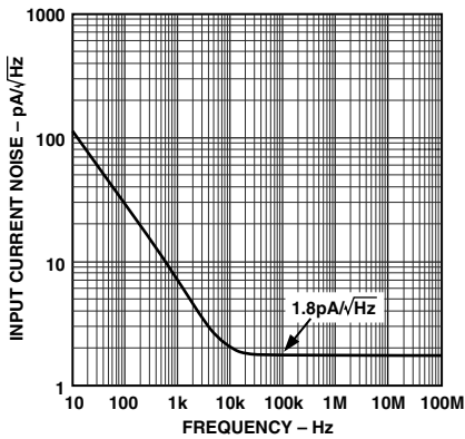
TPC 56. Input Current Noise vs. Frequency
