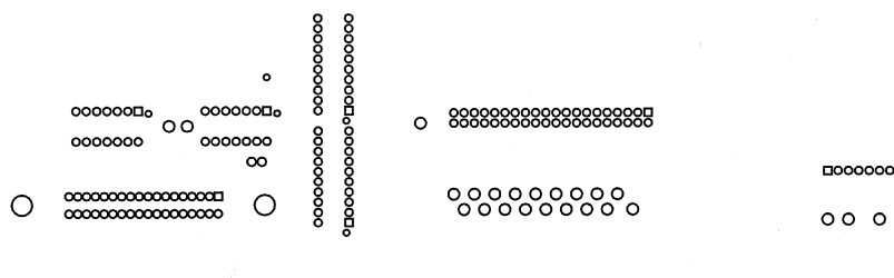
Figure 46. Soldermask Bottom
