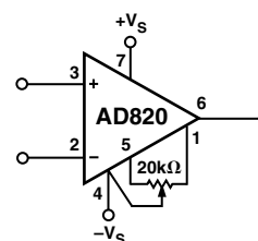
Figure 19. Offset Null
