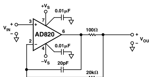
Figure 18. Extending Unity Gain Follower Capacitive Load Capability Beyond 350 pF
