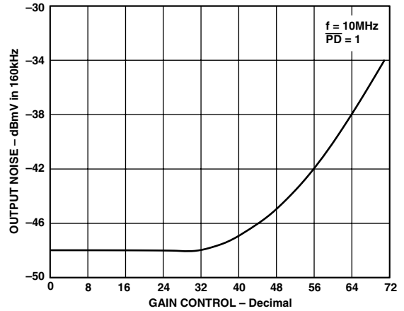
TPC 5. Output Referred Noise vs. Gain Control
