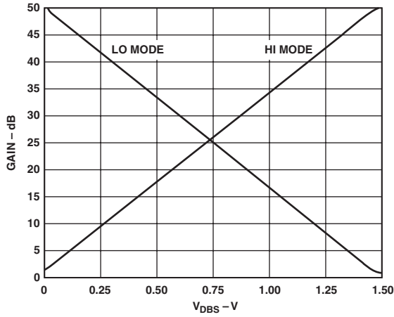
TPC 1. Gain vs. V_{DBS}
