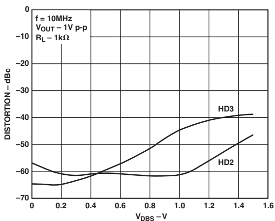
TPC 24. Harmonic Distortion vs. V_{DBS}
