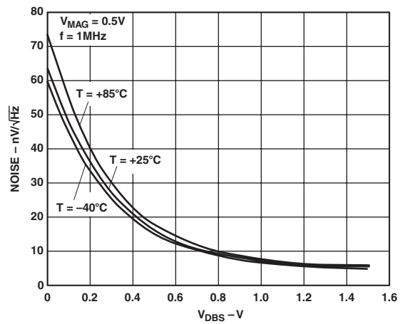
TPC 17. Input Referred Noise vs. V_{DBS} for Three Temperatures
