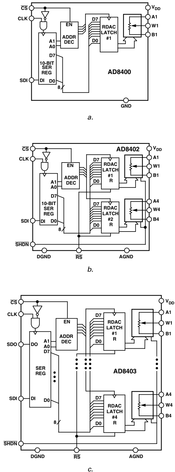
Figure 4. Block Diagrams
