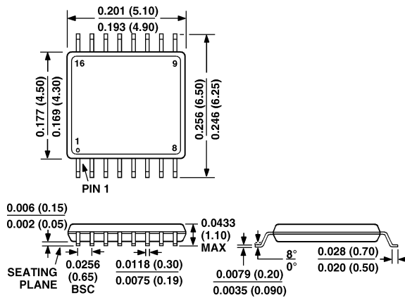
16-Lead Thin Shrink Small Outline (TSSOP) (RU-16)
