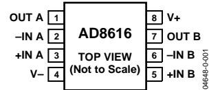
Figure 1. 8-Lead MSOP (RM-8)
