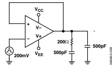
Figure 40. Snubber Network
