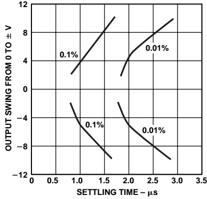
Figure 2. Settling Time
