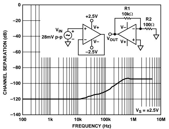
Figure 52. Channel Separation
