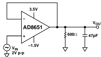
Figure 58. THD + N Test Circuit
