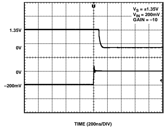
Figure 45. Negative Overload Recovery Time
