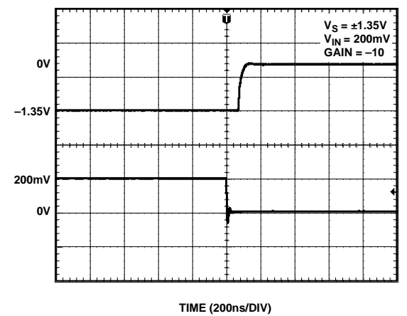
Figure 46. Positive Overload Recovery Time
