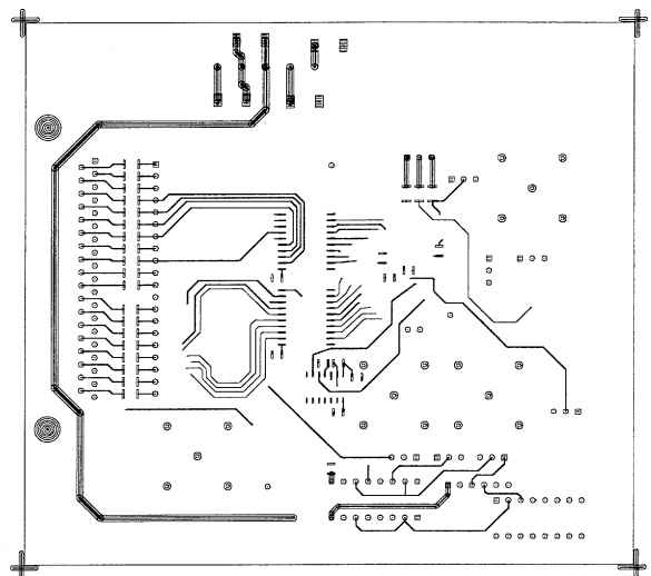
Figure 42. Conductors—Bottom View
