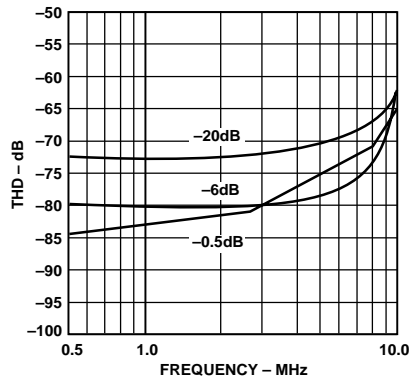
Figure 24. THD vs. Input Frequency (Input Span = 2.0 V p-p, V CM = 2.5 V)
