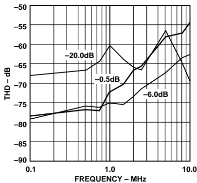
Figure 26. THD vs. Input Frequency (Input Span = 5.0 V p-p, V CM = 2.5 V)
