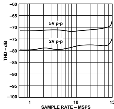
Figure 27. THD vs. Clock Frequency (A IN = -0.5 dB, f IN = 1.0 MHz, V CM = 2.5 V)
