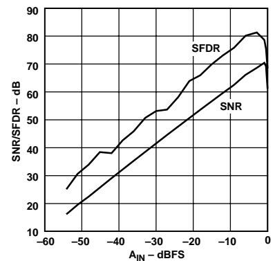
Figure 28. SNR/SFDR vs. A IN (Input Amplitude) (f IN = 5.0 MHz, Input Span = 2 V p-p, V CM = 2.5 V)
