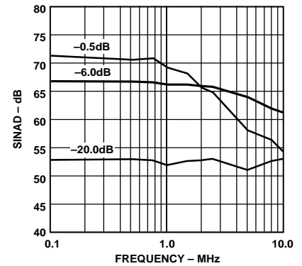
Figure 25. SINAD vs. Input Frequency (Input Span = 5.0 V p-p, V CM = 2.5 V)
