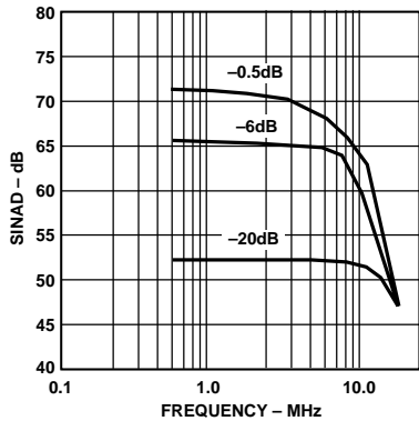
Figure 23. SINAD vs. Input Frequency (Input Span = 2.0 V p-p, V CM = 2.5 V)
