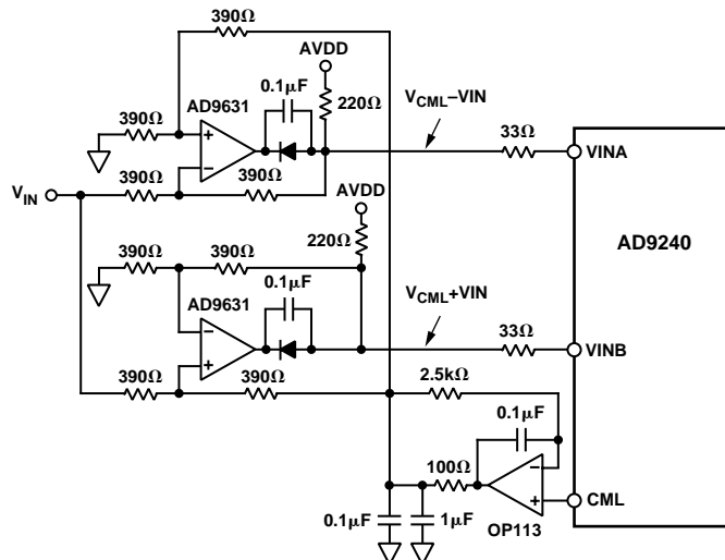
Figure 34. Differential Driver with Level-Shifting
