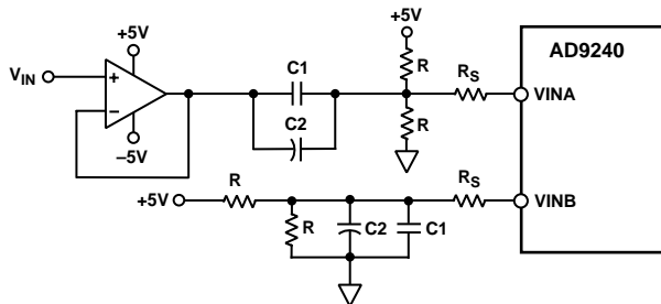
Figure 38. AC-Coupled Input-Flexible Input Span, V_{CM} = 2.5\text{ V}
