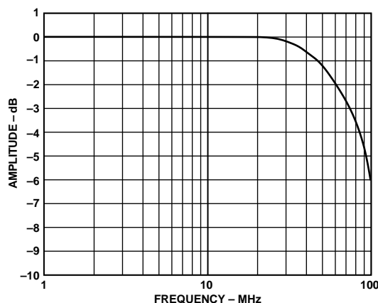
Figure 25. Full-Power Bandwidth
