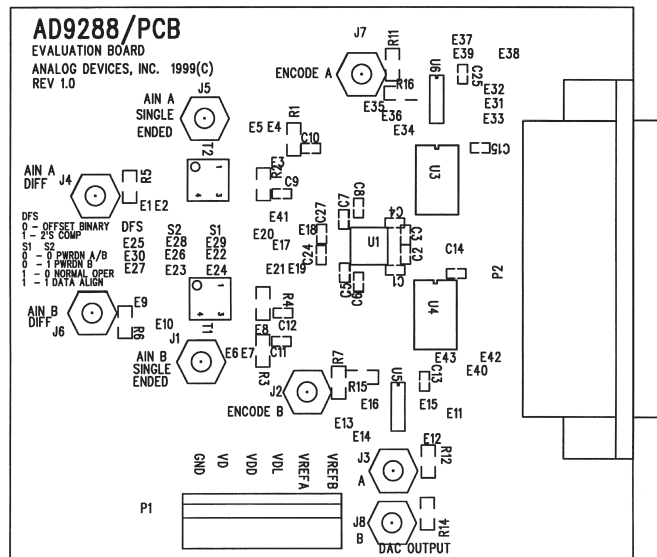
Figure 12. Printed Circuit Board Top Side Silkscreen
