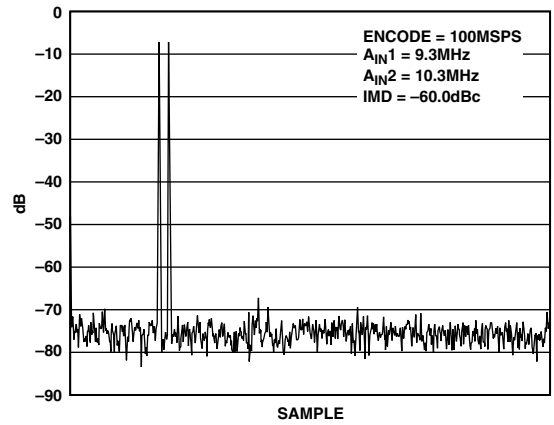
TPC 5. Two-Tone Intermodulation Distortion
