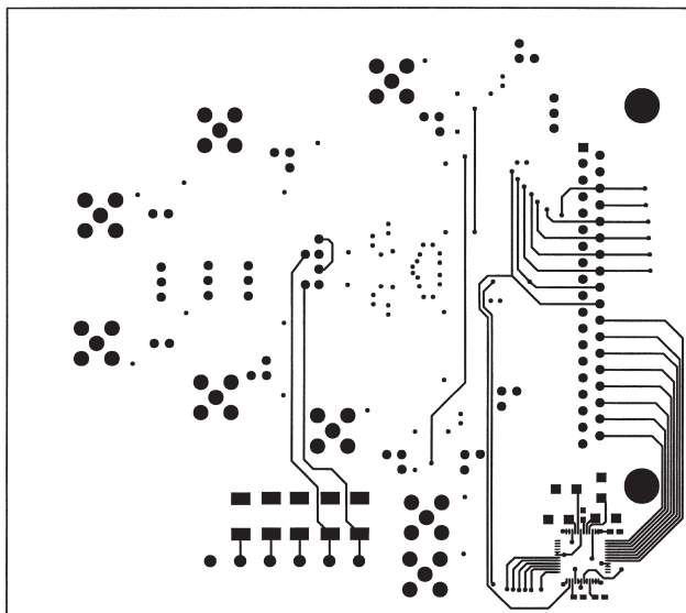
Figure 11. Printed Circuit Board Bottom Side Copper
