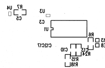
Figure 23. Bottom Silkscreen
