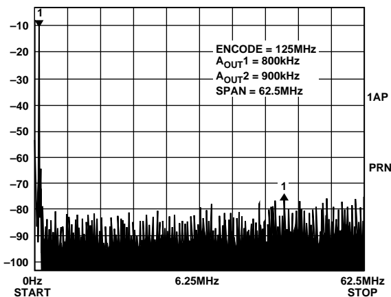
Figure 15. Wideband Intermodulation Distortion F_1 = 800 \text{ kHz} ; F_2 = 900 \text{ kHz} ; 125 \text{ MHz} Clock; \text{Span} = 62.5 \text{ MHz}
