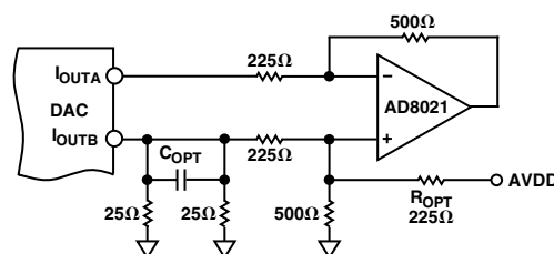
Figure 53. Op Amp-Coupled Output Circuit
