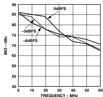
TPC 12. Third Order IMD Products vs. Two-Tone f_{OUT} @ f_{DATA} = 160\text{ MSPS}
