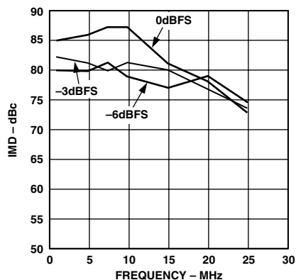
TPC 10. Third Order IMD Products vs. Two-Tone f_{OUT} @ f_{DATA} = 65\text{ MSPS}
