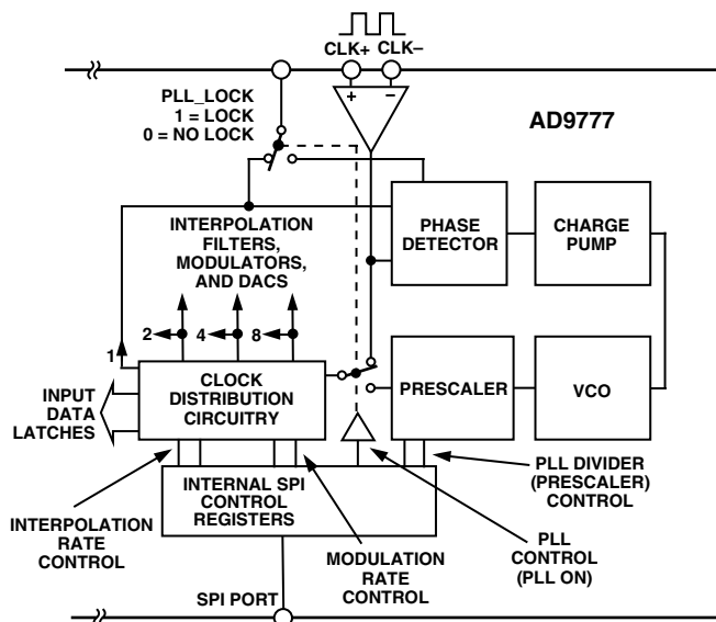
Figure 13. PLL and Clock Circuitry with PLL Disabled
