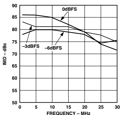
TPC 11. Third Order IMD Products vs. Two-Tone f_{OUT} @ f_{DATA} = 78\text{ MSPS}
