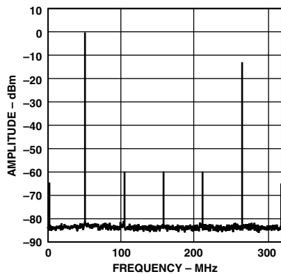
TPC 7. Single-Tone Spectrum @ f_{DATA} = 160\text{ MSPS} with f_{OUT} = f_{DATA}/3
