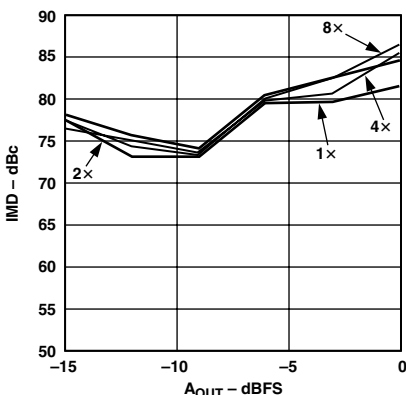
TPC 14. Third Order IMD Products vs. Two-Tone A_{OUT} and Interpolation Rate f_{DATA} = 50\text{ MSPS} for All Cases
