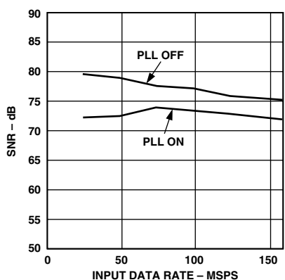
TPC 17. SNR vs. Data Rate for f_{OUT} = 5\text{ MHz}
