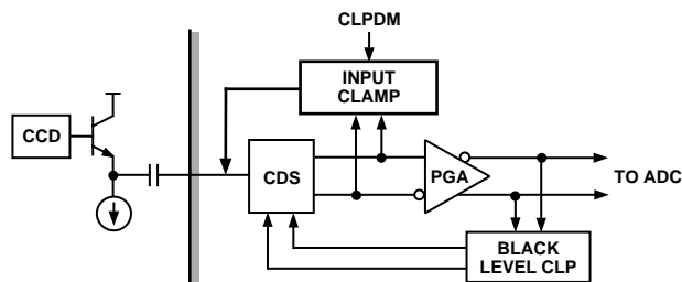
Figure 30. Input Clamp
