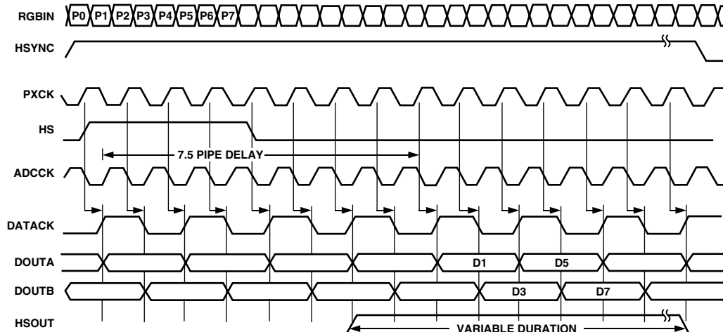
Figure 19. Dual-Channel Mode, Interleaved Outputs, Two Pixels/Clock (Odd Pixels)
