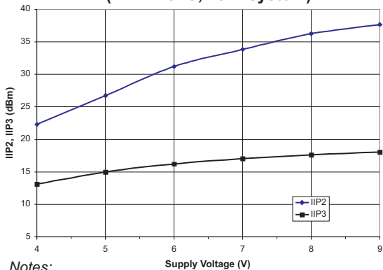
Figure 16: IIP2 and IIP3 vs. Supply Voltage - S24 Packaged Device (T A = +25 °C, 75 Ω system)
