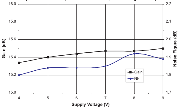
Figure 13: Gain and Noise Figure vs. Supply Voltage - S24 Packaged Device (T A = +25 °C, f = 500 MHz, 75 Ω system)
