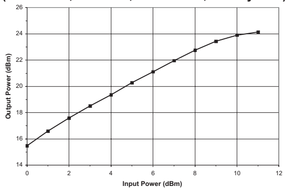
Figure 17: Output Power vs. Input Power S24 Packaged Device (T A = +25 °C, V DD = +8 V, f = 500 MHz, 75 Ω system)
