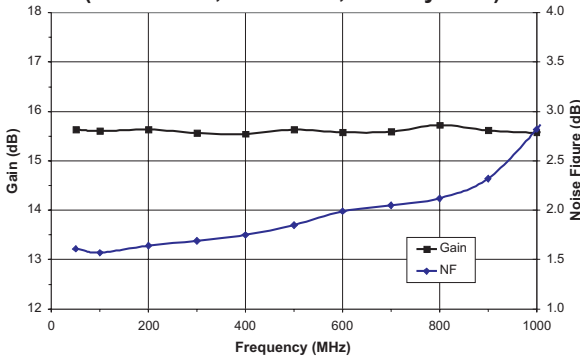
Figure 12: Gain and Noise Figure vs. Frequency - S24 Packaged Device (T A = +25 °C, V DD = +8 V, 75 Ω system)
