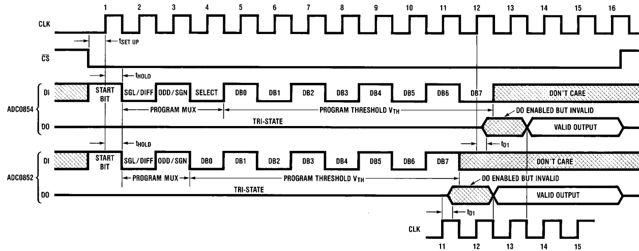
FIGURE 3. Timing Diagram
