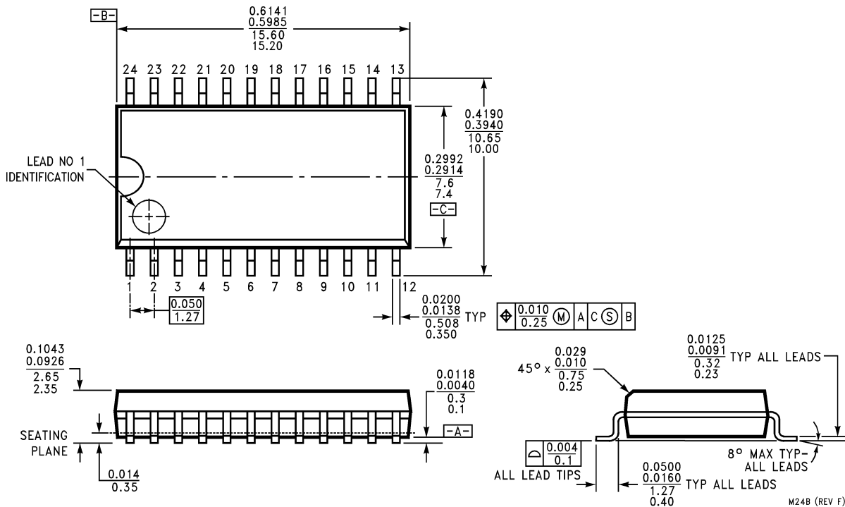
Order Number ADC10062CIWM NS Package Number M24B
