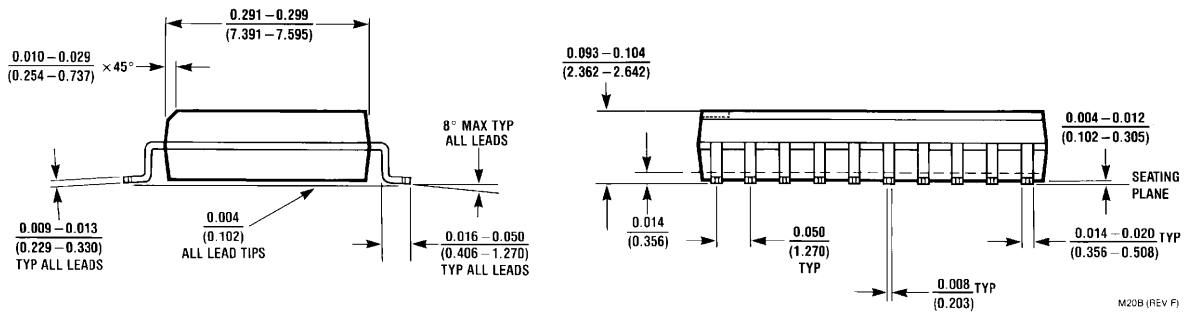
Order Number ADC10061CIWM NS Package Number M20B
