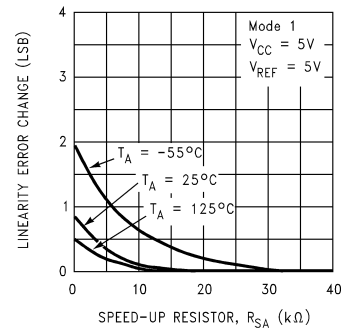
Linearity Change vs Speed-Up Resistor
