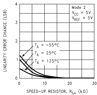
Linearity Change vs Speed-Up Resistor
