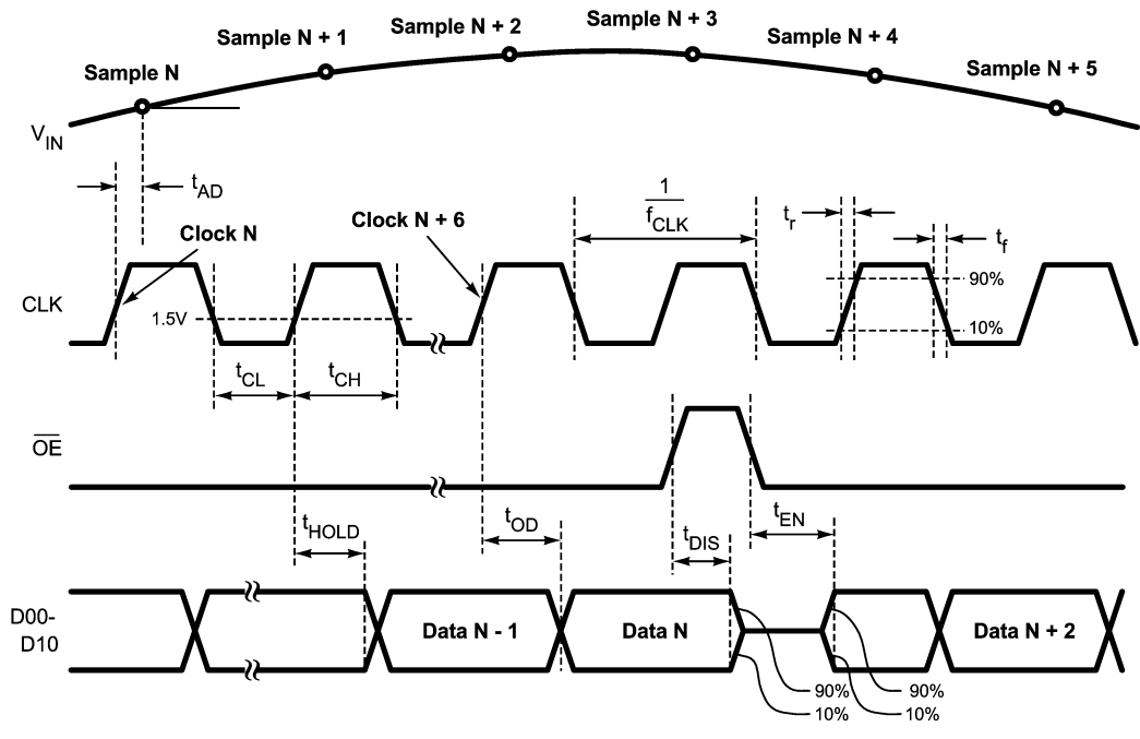
Output Timing
