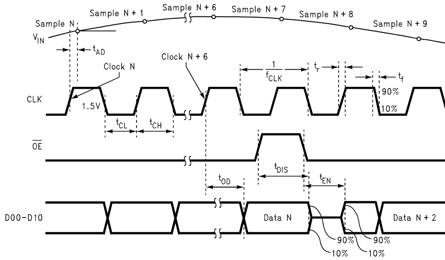
Output Timing
