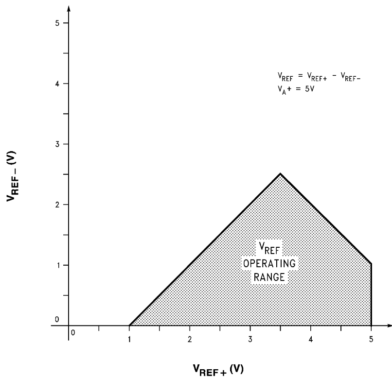
FIGURE 4. V_{REF} Operating Range for V_A = 5V
