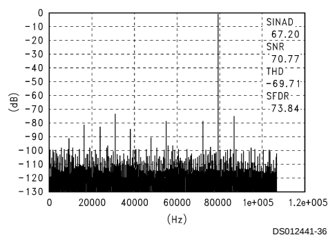
Full Scale Differential 79,468 Hz Sine Wave Input
