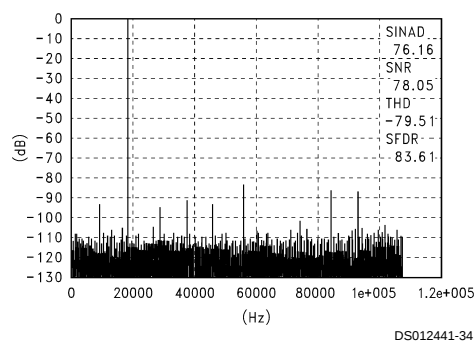
Full Scale Differential 18,677 Hz Sine Wave Input
