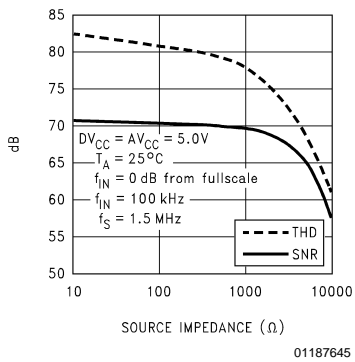
SNR and THD vs Source Impedance
