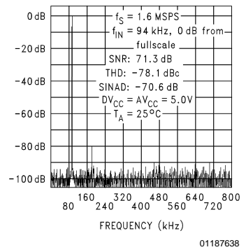
Spectral Response
