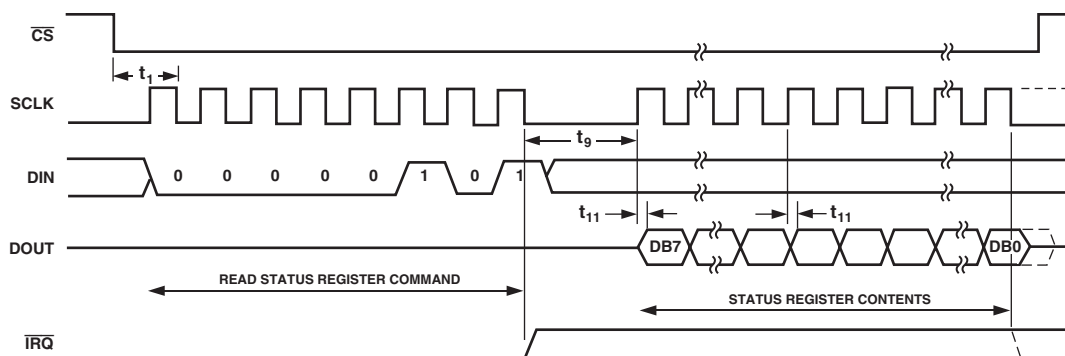
Figure 18. Interrupt Timing
