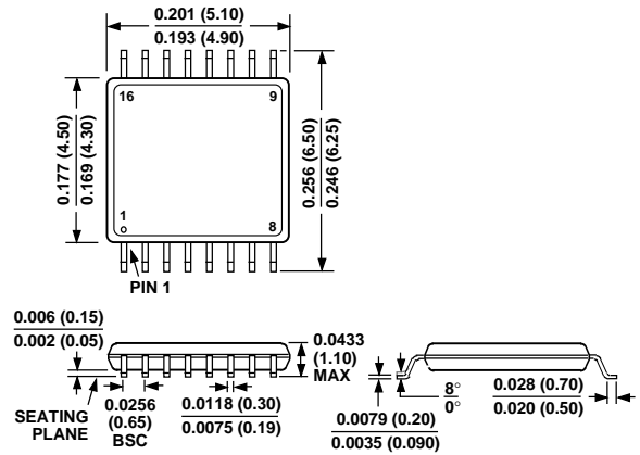
Thin Shrink Small Outline Package (TSSOP) (RU-16)
