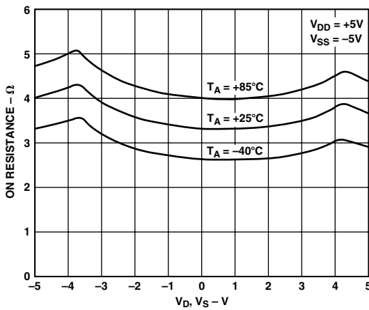
TPC 3. On Resistance vs. V_D (V_S) for Different Temperatures. (Dual Supply)
